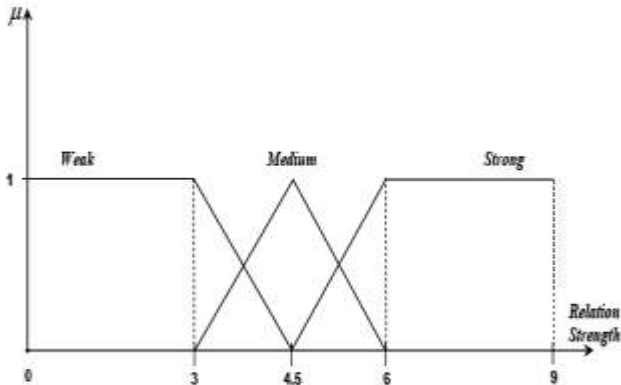
Figure-2 Illustration of the linguistic rules as fuzzy variables
